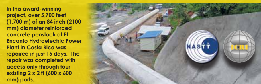
Equipment is delivered through access ports to avoid open cut trenches
