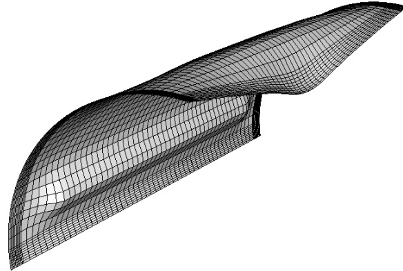
Figure 14. 3D simulation, imperfection, deformations
