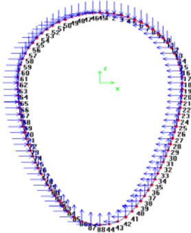
Figure 10a. Beam model for egg-shaped liners, loading
