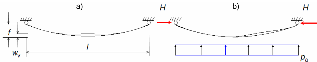
Figure 18a, b. Model of the invert shallow arch subjected to water pressure p_a , a) symmetric and b) non symmetric imperfection
