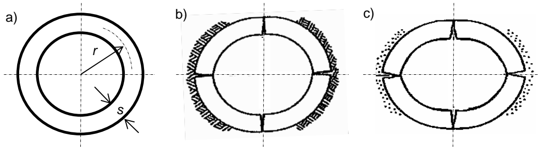
Figure 1a-c. Host pipe state I (a), II (b) and III (c) as defined in the German Design Code ATV-M 127-2
