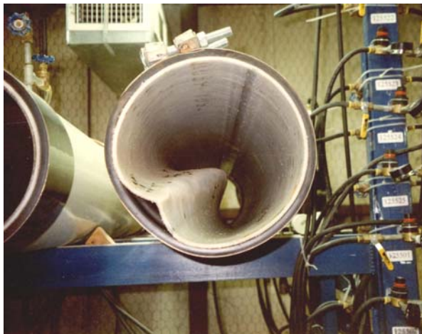
Figure 11. Long-term buckling tests on CIPP linings of the Louisiana Tech University (Guice et. al. 1994)
