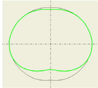
Figure 10b. Admissible deflection with one lobe in the invert
