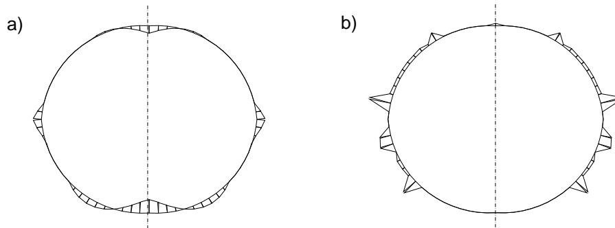
Figure 6a, b. Load cases groundwater p_a and soil pressure q_v – a system without horizontal symmetry, a) bending moments of the liner, b) contact forces liner versus host pipe (Linerb, 2007)
