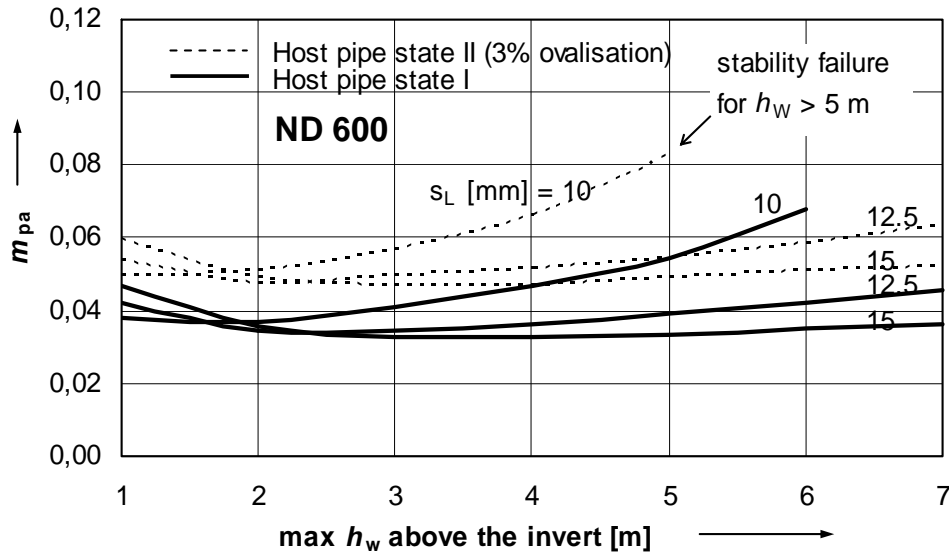
Figure 4. Invert bending moment factors for a lining with ND 600, source: Appendix A4 in M 127-2
