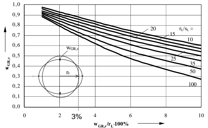
Figure 3a-c. Reduction factors \kappa_v , \kappa_s and \kappa_{GR,v} for the buckling pressure due to local imperfection w_v , annular gap w_s and global imperfection w_{GR,v} ; source: ATV-M 127-2:2000
