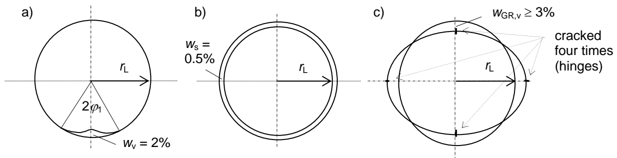
Figure 2a-c. Local imperfection w_v (a), annular gap w_s (b), global imperfection w_{GR,v} (c), minimum values
