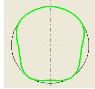
Figure 10c. Not acceptable multi-lobe figure for host pipe state I
