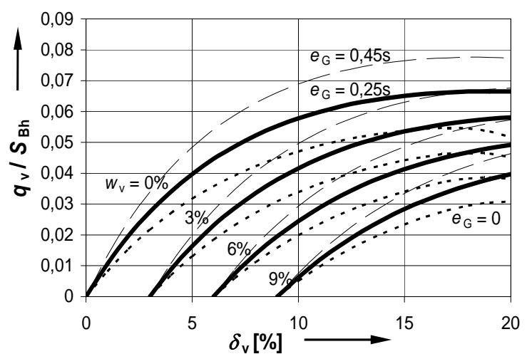
Figure 9. Load deflection-curves of the pipe soil-system for soil group 1, varying imperfections + hinge excentricities e_G
