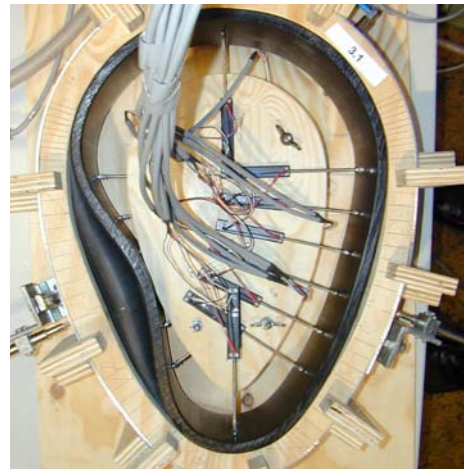
Figure 12. Creep buckling tests on egg-shaped PE linings, University of Applied Sciences Münster (Falter, 2008)
