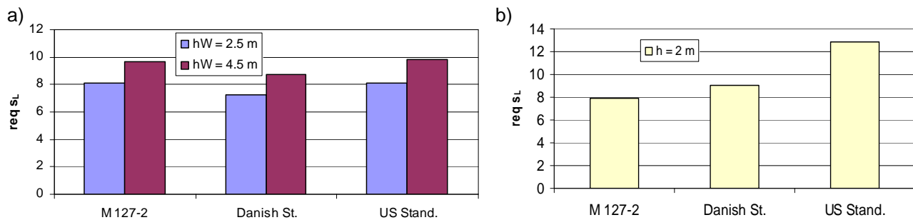
Figure 23a, b. Comparison of the required wall thickness of linings a) host pipe state I (water table h_w ) and b) host pipe state III (soil cover h and traffic load)
