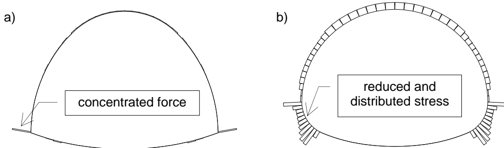
Figure 17a, b. Contact forces between polycrystalline liner and grout, a) sharp edges and b) rounded edges
