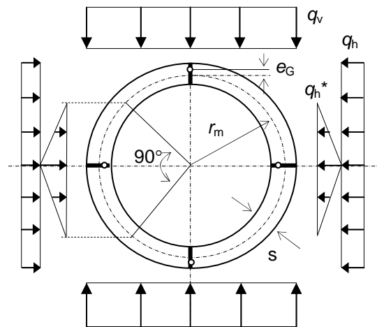
Figure 8. Pipe with longitudinal cracks and soil pressures q_v , q_h and q_h^* (support)
