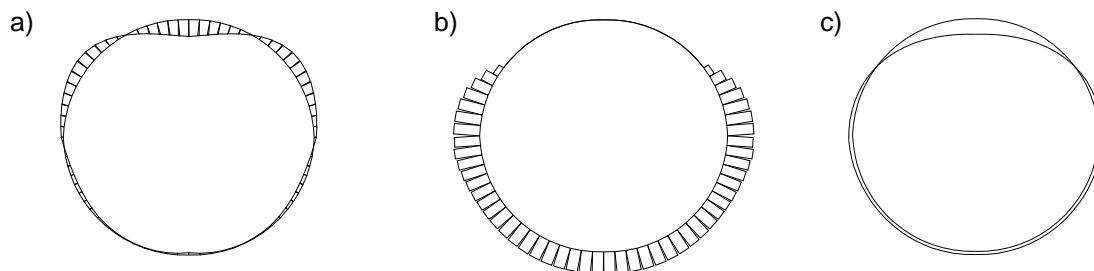
Figure 7a-c. Bending moments (a), contact forces (b) and deflections (c) of a circular lining subjected to groundwater - host pipe neglected (Linerb, 2007)
