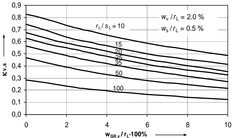
Figure 5. Reduction factors \kappa_{v,s} of the buckling pressure, 2% local imperfection, 0.5 % annular gap and arbitrary global imperfection (Falter, 2003)
