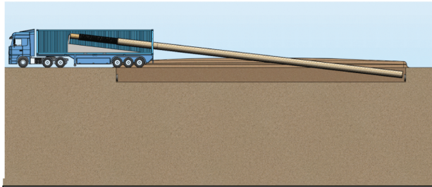
Pipeline of nearly any shape or diameter can be produced at a job site in lengths up to 1,000 ft without joints using a new process that sandwiches a durable but lightweight honeycomb material between two layers of resin-saturated carbon-fiber fabric. © PipeMedic, LLC/Graphic by Reynard Perrin and Joerg Schmit
